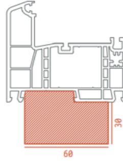
U=0,65 W/m 2 K Rehau Geneo
