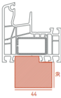
U=0,88 W/m 2 K Aluplast Ideal 5000, Ideal 4000
